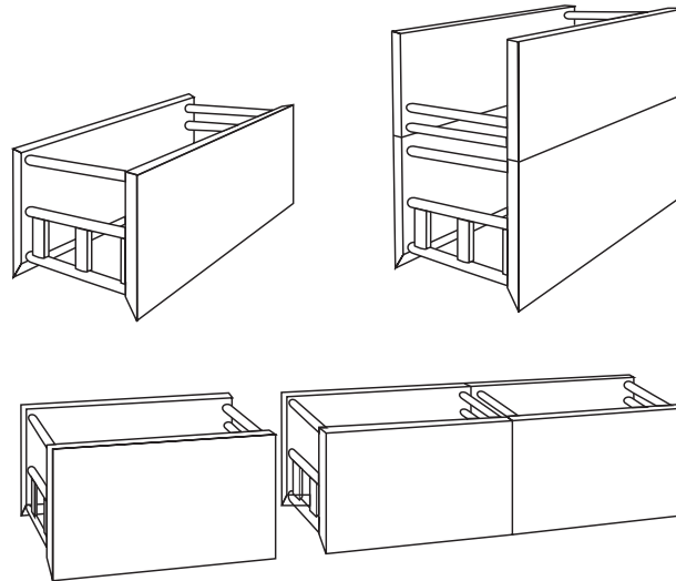
Figure 2. Trench Shields
